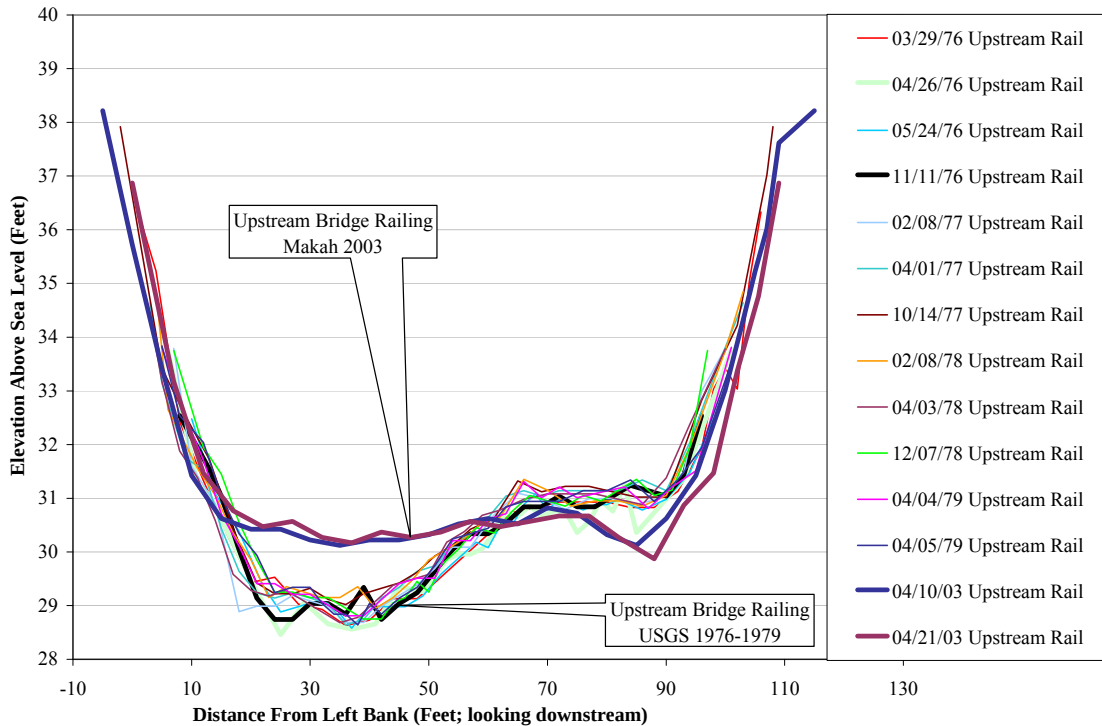
Figure 4.38. Cross-section elevation data collected from the upstream bridge railing on the Ozette River (source: USGS; MFM, unpublished data).
