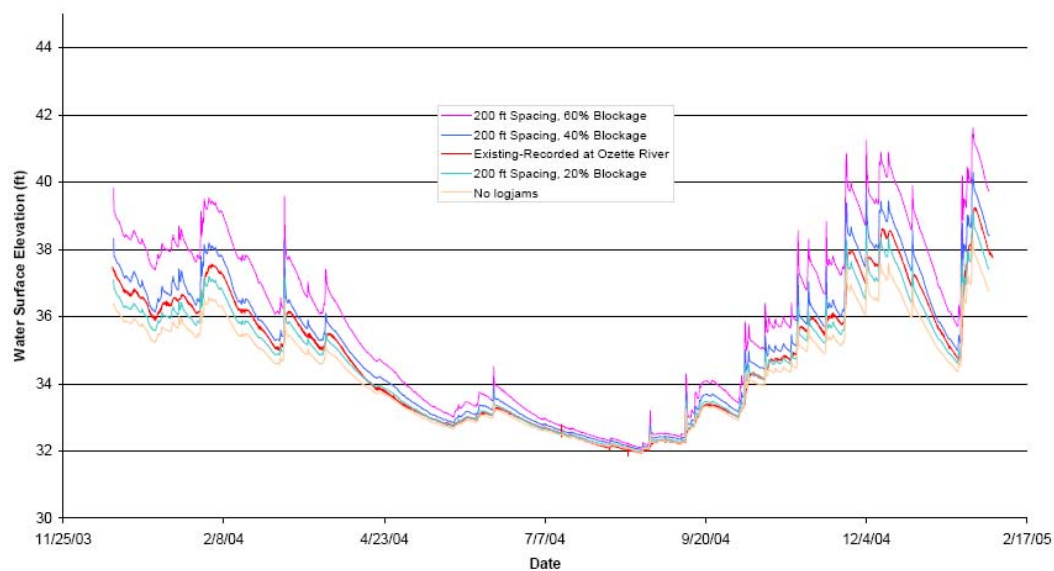
Figure 5.5. Comparison of modeled water surface elevations at the lake's outlet for existing conditions, no jams, and 200-foot spacing at 20, 40, and 60 percent blockage (source: Herrera 2005).
