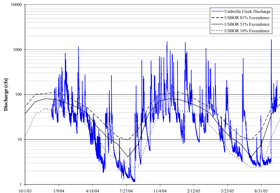
Figure 4.54. Provisional Umbrella Creek discharge data plotted with USBOR synthesized monthly average streamflow exceedence curves (source: MFM, unpublished data; Lieb and Perry 2004).
