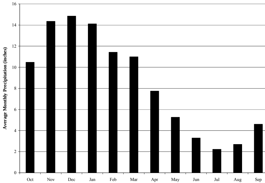
Figure 1.5. Average monthly precipitation for Quillayute Airport weather station WY 1967 to WY 2005 (source: NOAA-NCDC 2005)
