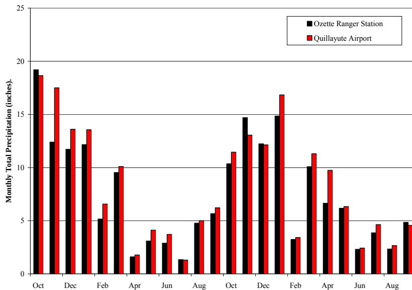
Figure 1.7. Monthly rainfall comparison, Quillayute versus Ozette for WY 2004 and 2005 (source: NOAA-NCDC 2005; ONP, unpublished data).
