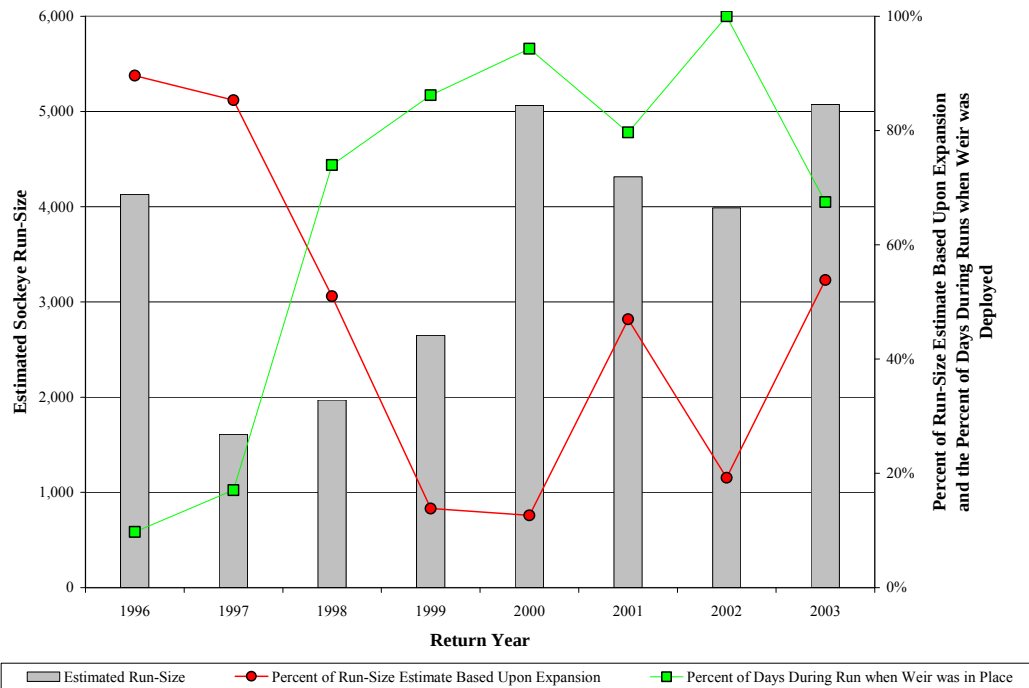
Figure 3.23. Estimated Lake Ozette sockeye run sizes for return years 1996 to 2003 contrasted with the proportion of the run-size estimates that were based upon expansion and the percentage of run-days in which the weir was deployed (source: Haggerty 2004a, 2005a, 2005b, 2005c, 2005d).
