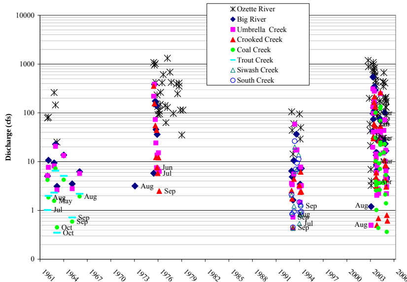
Figure 4.33. Instantaneous stream discharge measurements (source: USGS, Meyer and Brenkman 2001; MFM, unpublished discharge data).
