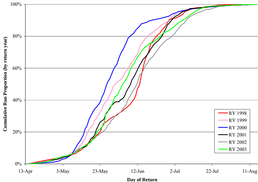
Figure 3.3. Observed and estimated cumulative run proportion by return year for years 1998 through 2003 (source: Haggerty 2005d).
