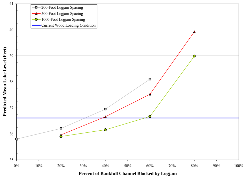
Figure 5.26. Comparison of observed mean lake level for October 15, 2004 through January 30, 2005 and different wood loading scenarios in the Ozette River and their corresponding predicted mean lake levels (modified from Herrera 2005). Note that this predicted mean lake level was for the modeled spawning period (October 15, 2004 to January 30, 2005), and does not correspond to the long-term measured mean lake level of 34 feet (Section 4.3.5).
