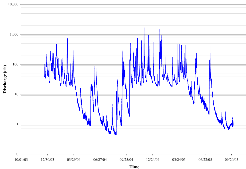
Figure 4.73. Provisional Crooked Creek discharge data (source: MFM, unpublished data).
