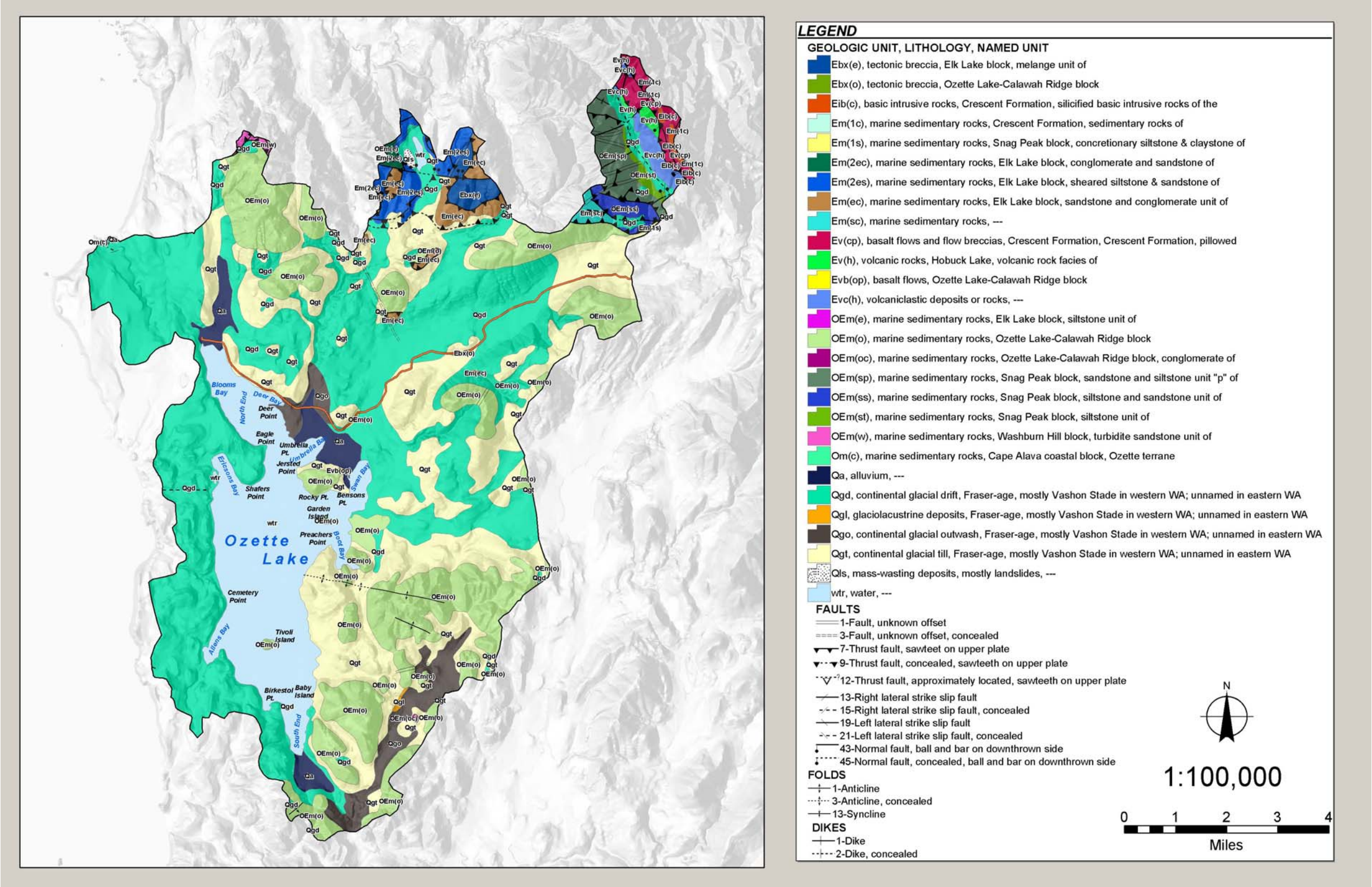
Figure 1.3. Ozette watershed geology (source: Schasse2003)
