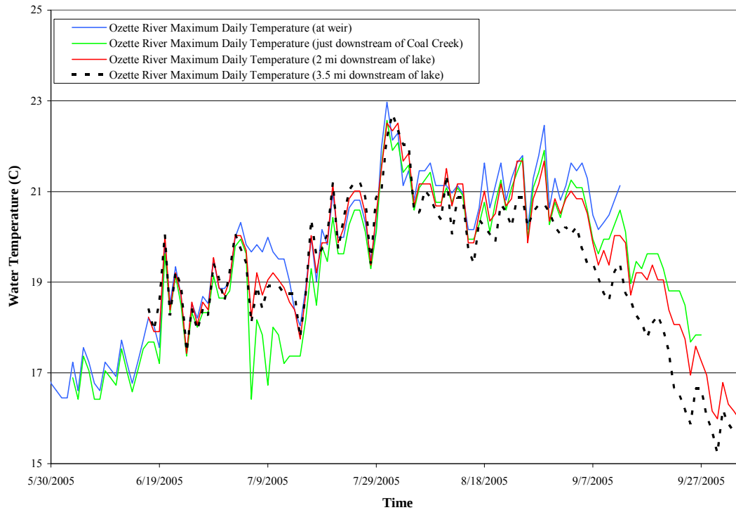
Figure 4.32. Ozette River daily maximum temperature at the Ozette counting weir, just downstream of Coal Creek, 2 miles downstream of lake, and 3.5 miles downstream of lake (source: MFM unpublished data).
