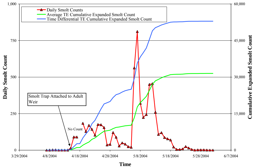
Figure 3.20. Ozette River daily sockeye smolt counts, average trap efficiency expanded cumulative sockeye smolt counts, and time differential trap efficiency expanded cumulative smolt counts, spring 2004 (source: Peterschmidt 2005)
